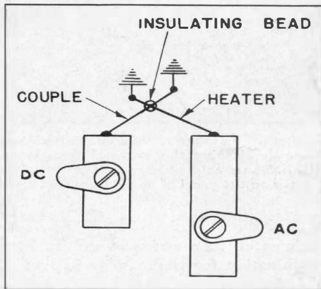
FIGURE 3b. Sketch showing the arrangement of the elements.
