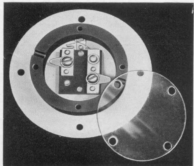
FIGURE 2. Rear view of the thermocouple.
