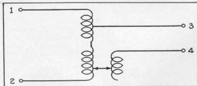
FIGURE 2. (Left) Connections for TYPE 70-A2 and TYPE 80-A2. The input terminals are numbered 1-2; the output terminals 3-4. (Right) Connections for TYPE 70-B2, TYPE 80-B2, and TYPE 80-C2. Input is applied at terminals 3-4 and the output appears at 1-2.
