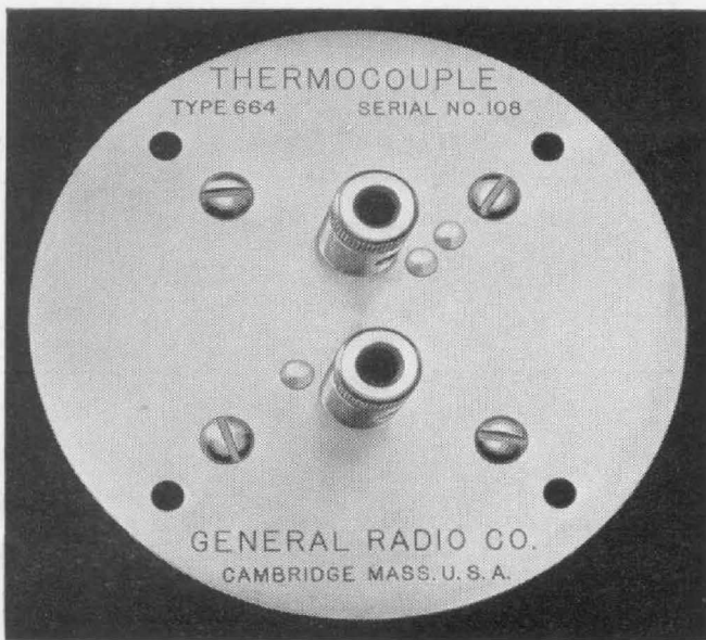
FIGURE 1. Front view of the TYPE 664-A Thermocouple showing the standard-voltage terminals. The circular plate mounts in the shield or on the panel of an r-f generator.
